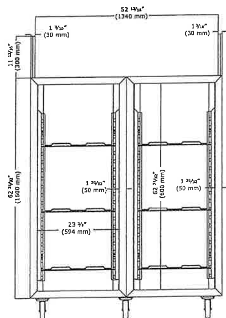
Front (Open)
