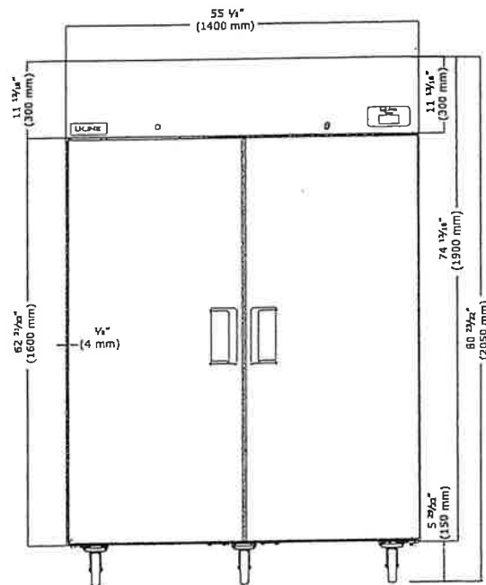
Front (Closed)
