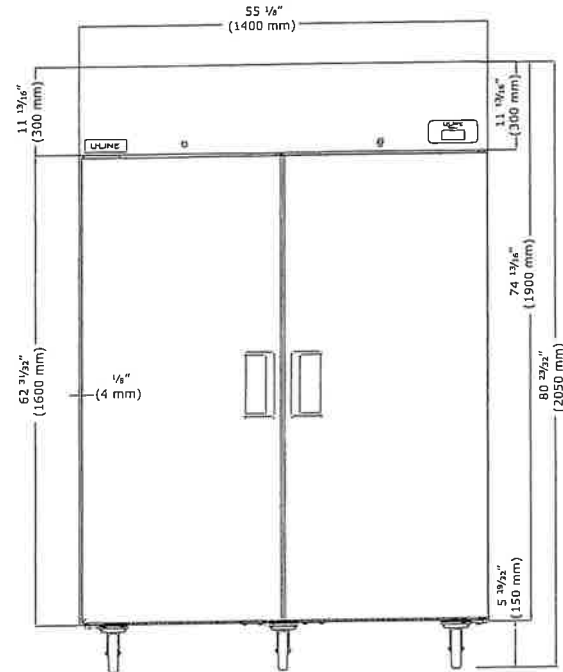
Front (Closed)
