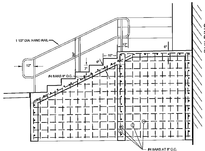
STAIR SECTION B-B
