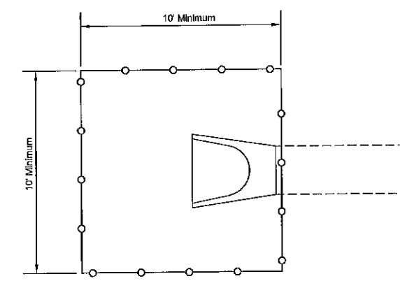
SILT FENCE AT DRAINAGE STRUCTURE NO SCALE
