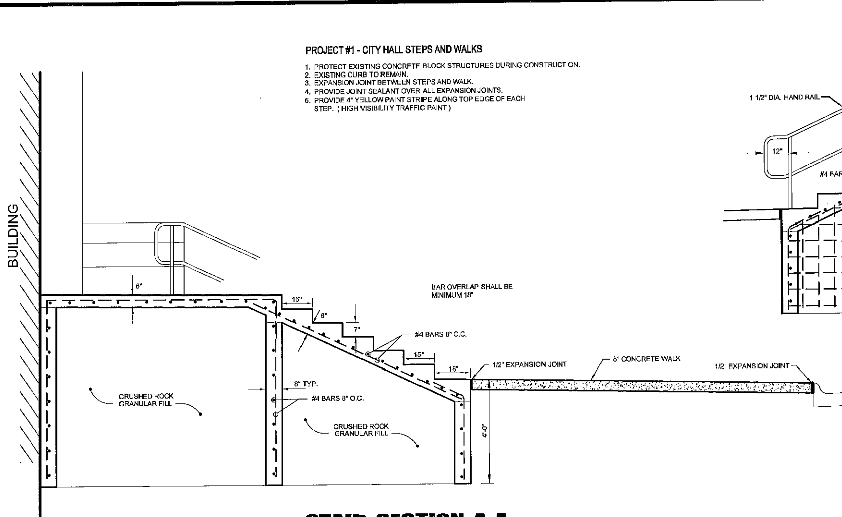
STAIR SECTION A-A
